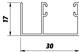
BOXIN-CA010 0,210kg/m
