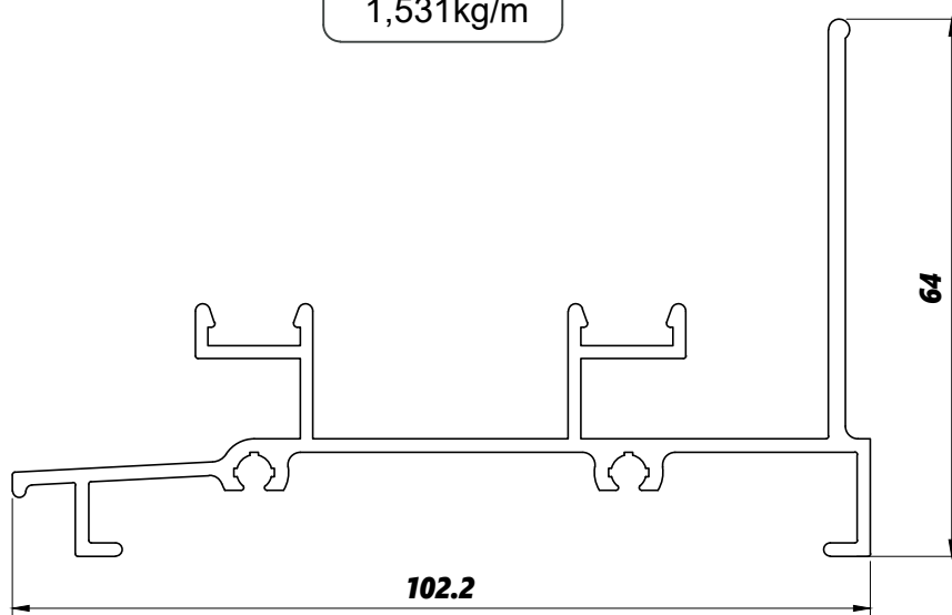
LG115 1,241kg/m
