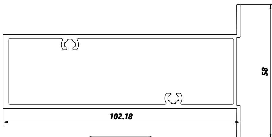
LG176 1,499kg/m
